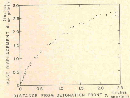
FIG. 3. Example of typical experimental data of image displacement versus distance behind the detonation front.
